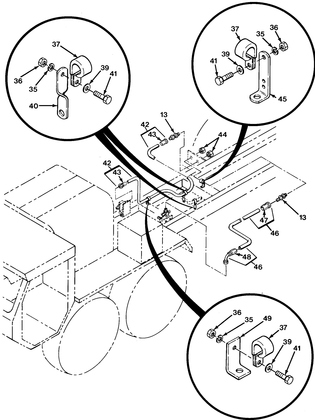
FIG.417 HYDRAULIC LINES AND FITTINGS - M983 WITHOUT CRANE (SHEET 3 OF 3)
