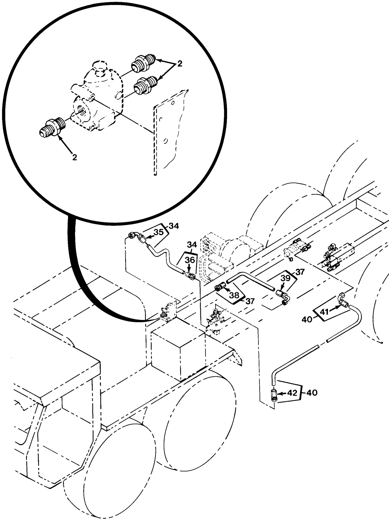
FIG.415 HYDRAULIC LINES AND FITTINGS - M978 WITH WINCH (SHEET 2 OF 4)
