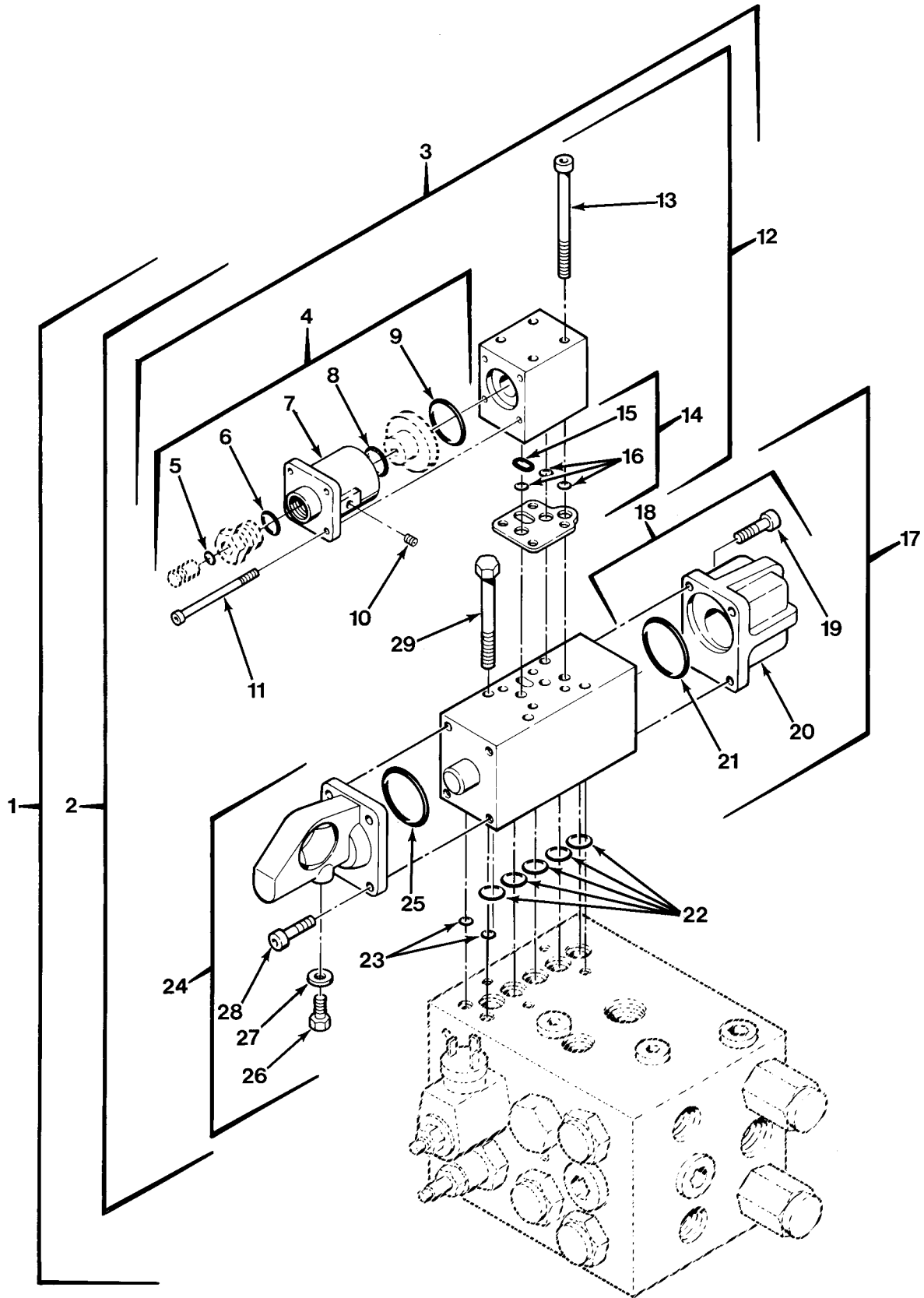
FIG.410 HEAVY DUTY WINCH MANIFOLD -M984A1 (SHEET 1 OF 3)
