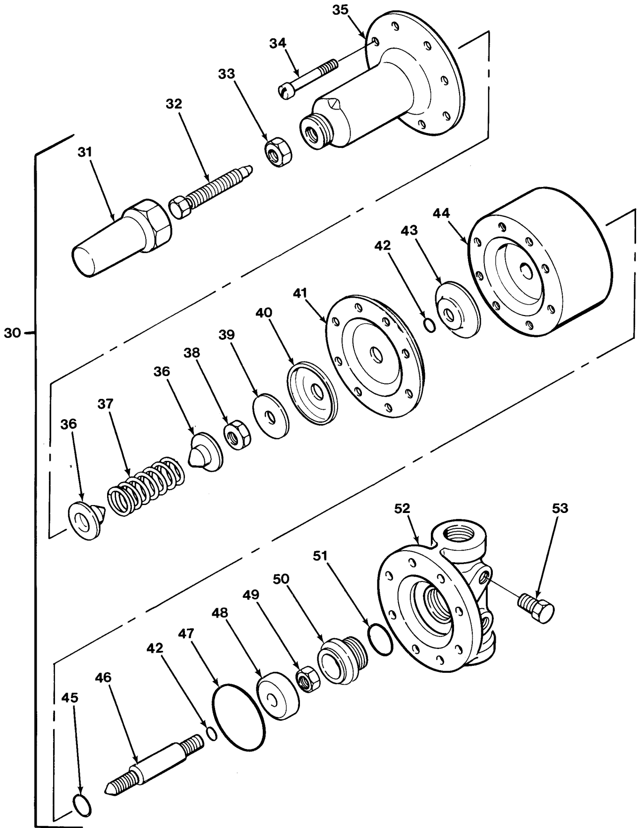
FIG.470 V4 RELIEF VALVE (SHEET 2 OF 3)
