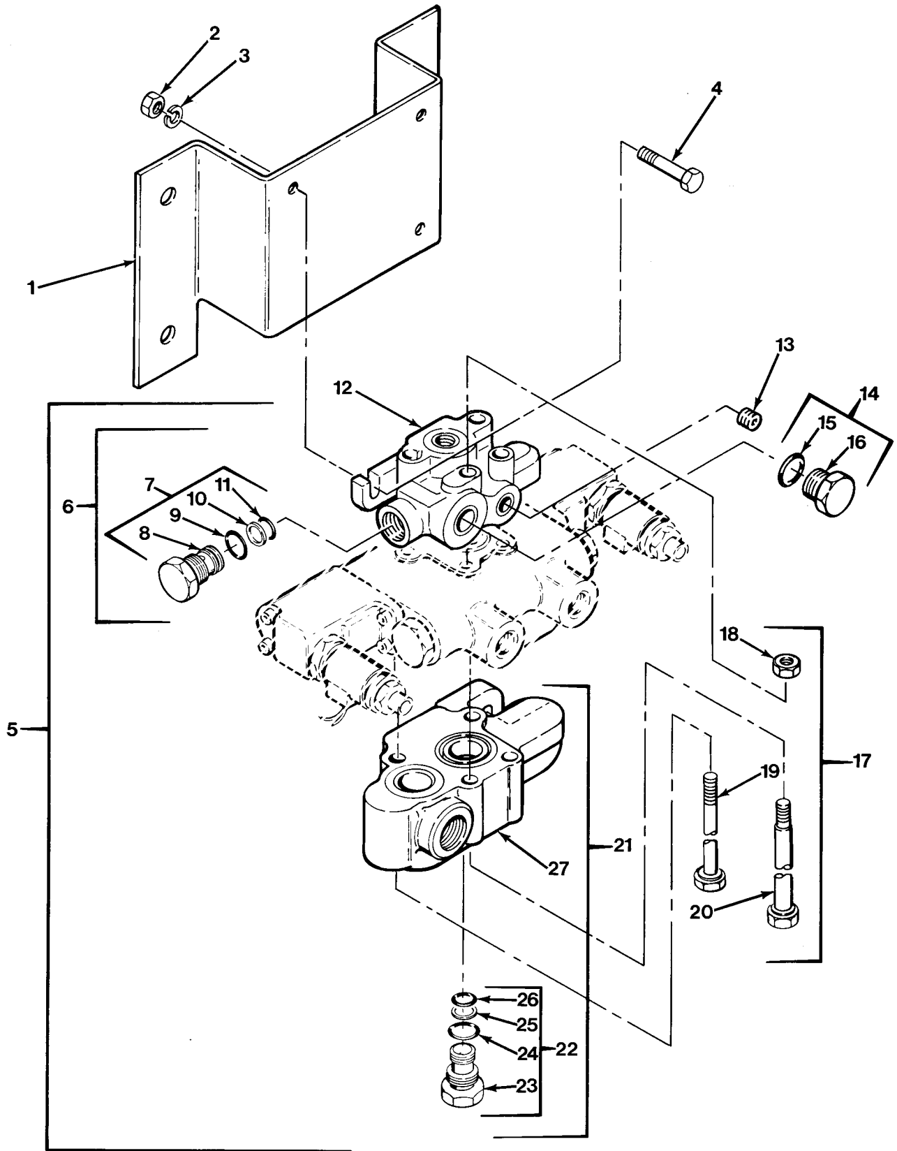
FIG.408 HEAVY DUTY WINCH SELECTOR VALVE - M984 (SHEET 1 OF 2)
