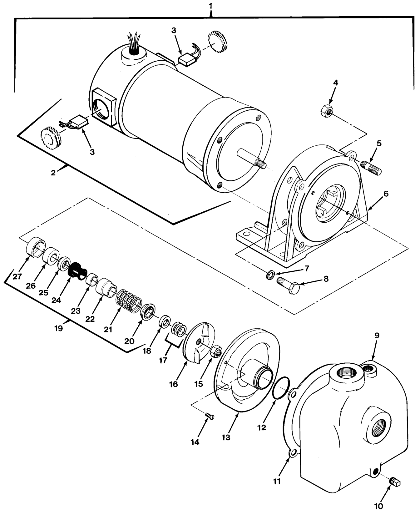
FIG.444 AUXILIARY PUMP
