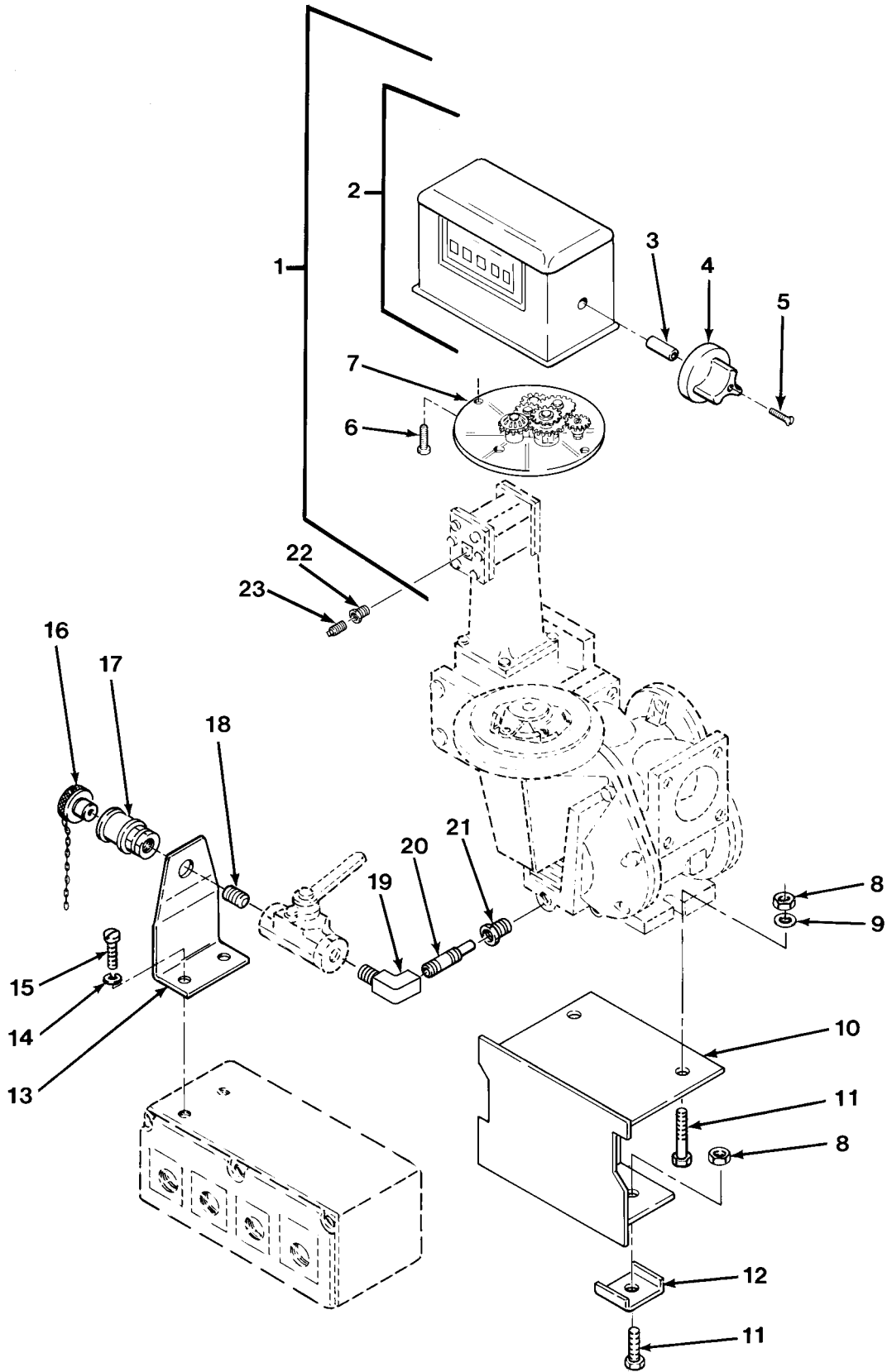
FIG.445 FLOWMETER INSTALLATION
