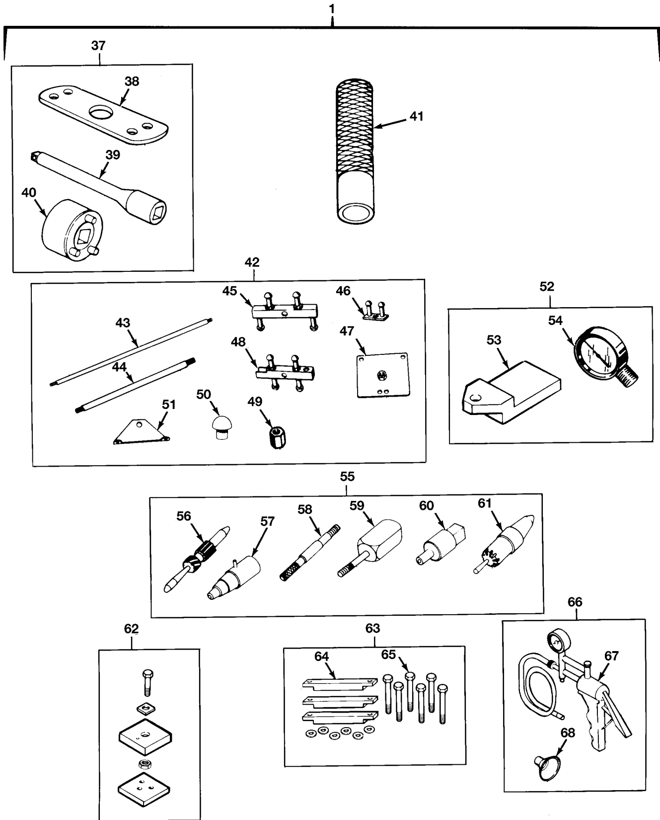
FIG.476 GENERAL SUPPORT SPECIAL TOOLS (SHEET 4 OF 8)
